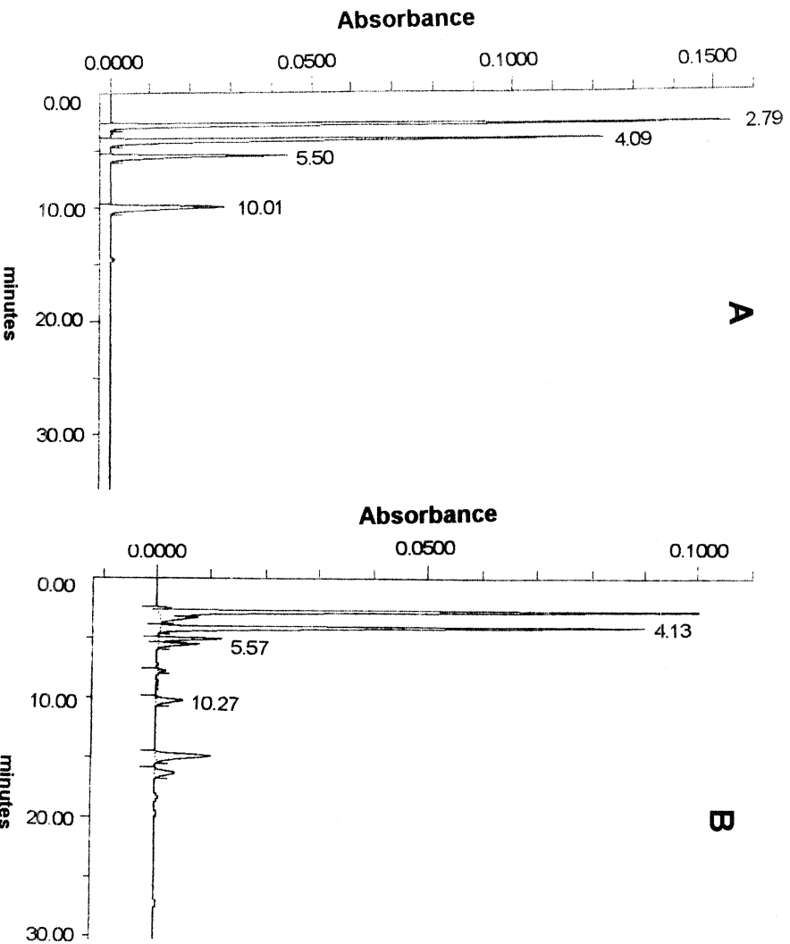
Fig. 5. Chromatograms of 1% solutions of a pharmaceutical preparation containing caffeine, 8-chlorotheophylline and diphenhydramine as active principles submitted to oxidative stress. Conditions: SymmetryShield RP8 column, acetonitrile–(0.01 M H 3 PO 4 –triethylamine, pH 2.8) (22:78, v/v), flow-rate of 1 ml/min and UV detection at 229 nm. (A) Before decomposition; (B) after 1 h heating with 0.3% H 2 O 2 in an autoclave at 120°C.
