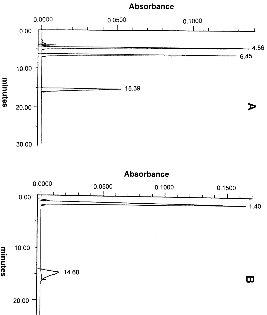
Fig. 3. Chromatograms of standards of caffeine, 8-chlorotheophylline and diphenhydramine in acetonitrile–(0.01 M H_3PO_4 –triethylamine pH, 3.0) (20:80, v/v) at a flow-rate of 1 ml/min and UV detection at 229 nm. (A) in a SymmetryShield RP8 column; (B) in a Nova-Pak C_{18} column.
