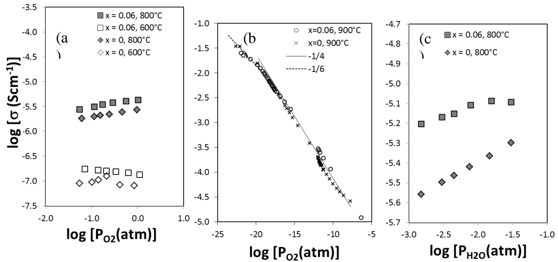
Fig. 7. Selected partial-pressure dependencies of electrical conductivity for \text{Sr}_3\text{NdNb}_{3-x}\text{Ti}_x\text{O}_{12-\delta} ( x = 0 and 0.06 ): (a) bulk conductivity as a function of p_{\text{O}_2} in dry oxidising conditions; (b) total conductivity as a function of p_{\text{O}_2} in reducing conditions; (c) bulk conductivity as a function of p_{\text{H}_2\text{O}} in oxidising atmosphere.
