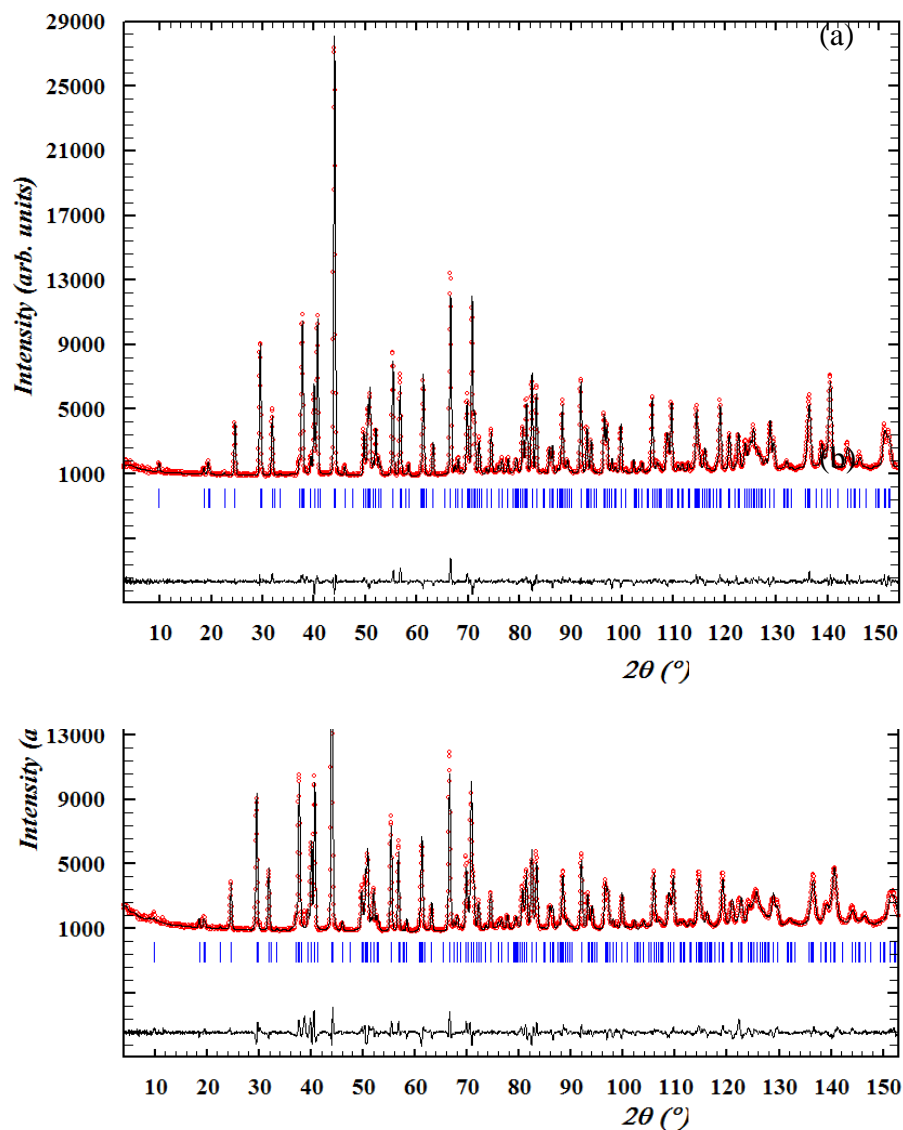
Fig. 3. Observed (circles), calculated (continuous line) and difference (continuous line at bottom) neutron powder diffraction profiles of (a) \text{Sr}_3\text{NdNb}_3\text{O}_{12} and \text{Sr}_3\text{NdNb}_{2.94}\text{Ti}_{0.06}\text{O}_{12-\delta} . Vertical bars indicate the expected position of Bragg peaks.
