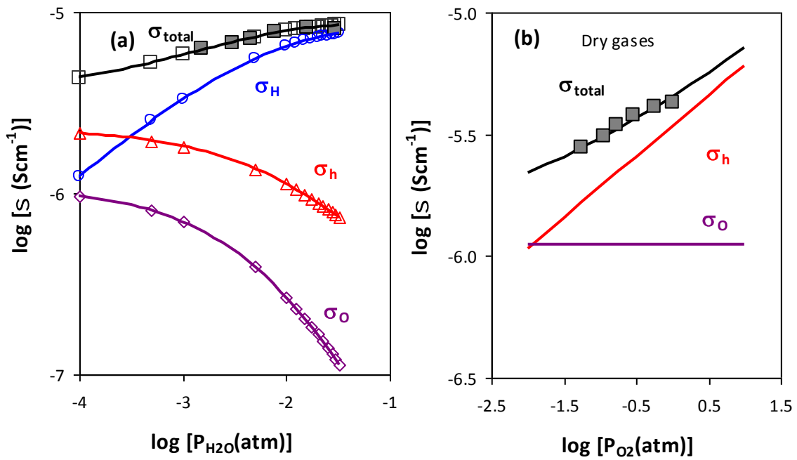
Fig. 9. Simulated conductivity profiles of transport species and total conductivity as a function of (a) p H 2 O and (b) p O 2 showing fit with the experimental results of total conductivity (closed squares) for Sr 3 NdNb 2.94 Ti 0.06 O 12-δ .
