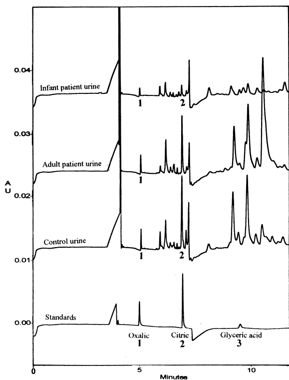
Fig. 1. Electropherograms of standards (oxalic, citric and glyceric acids), control urine, urine from adult and urine from an infant patient analysed by CE using buffer S. Applied voltage, -10 kV; injection for 5 s; pressure, 0.5 p.s.i. (see Section 2).
