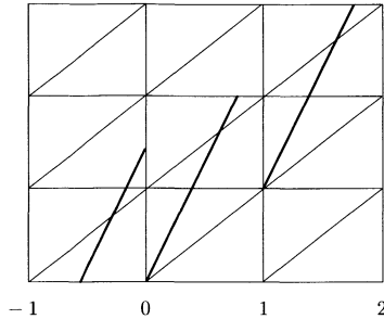
Figure 2. A Lorenz-like map.
