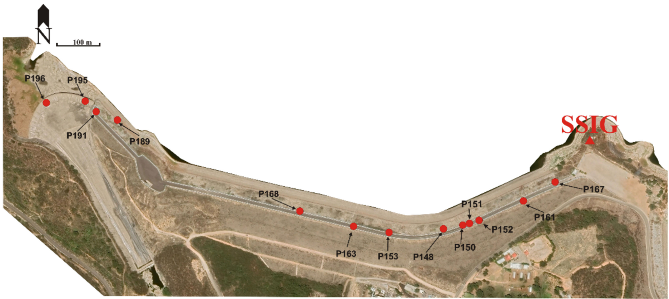
Figure 7. Location of the 13 PSs identified along the Sanalona dam in the MT-InSAR analysis.
