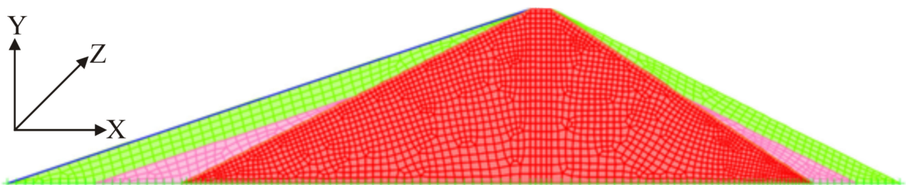
Figure 3. Cross-section FEM model of the Sanalona dam.
