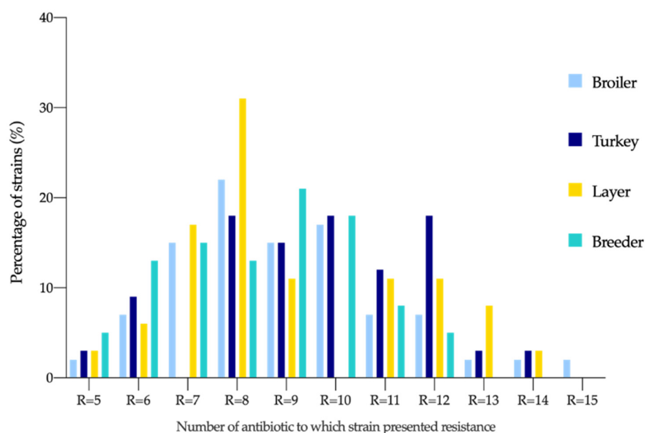
Figure 1. Resistance distribution according to different poultry production types. R = Number of antimicrobial resistances.
