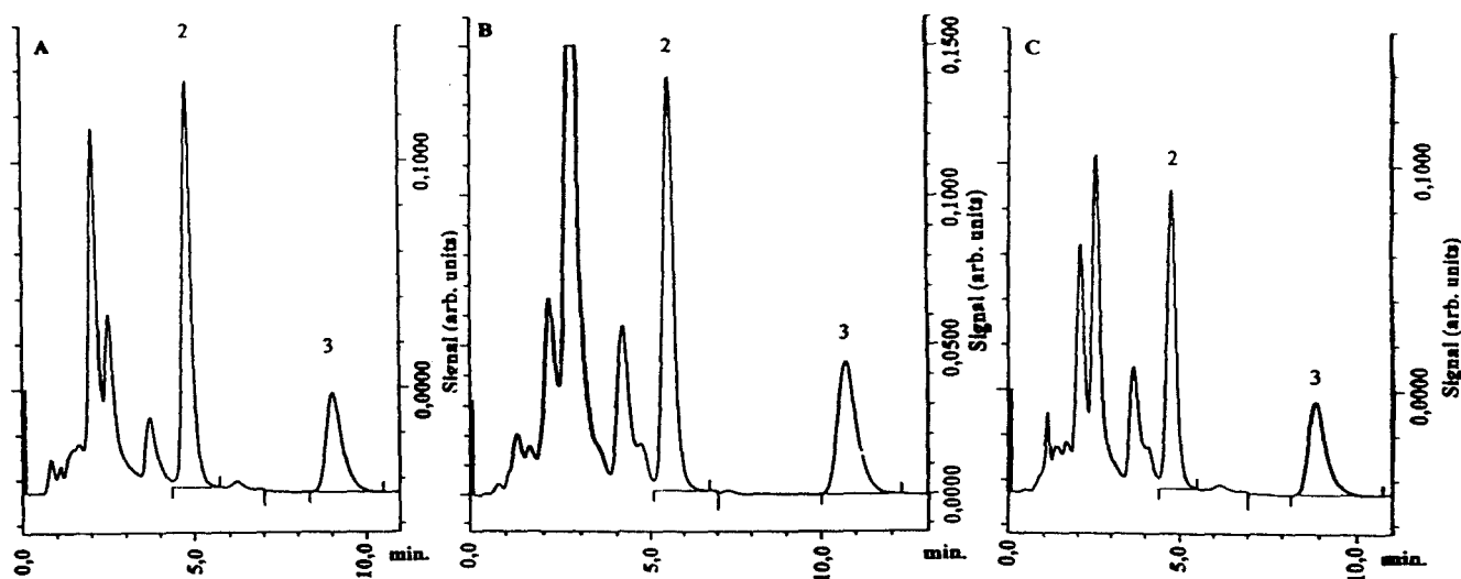
Fig. 2. Chromatograms corresponding to (A) standards; (B) placenta tissue extract; (C) brain tissue extract, all of them with fluorescent detection. Peak identification: 2: vit. E, 3: vit. K.
