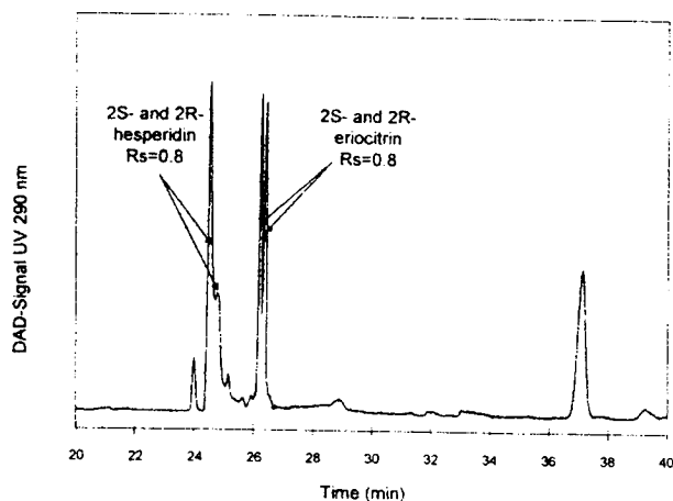
Figure 4. Chiral separation of 2 S - and 2 R -diastereomers of eryocitrin and hesperidin in lemon juice. Running buffer, 0.2 M borate buffer, 5 mM \gamma -CD at pH 10.0. Uncoated fused-silica capillary, l_t = 67 cm, l_d = 60 cm, 75 \mu m ID. Capillary temperature, 25°C. Run voltage, 15 kV. Injection at 0.5 psi for 2 s. UV detection at 290 nm. Reprinted from [79], with permission.
